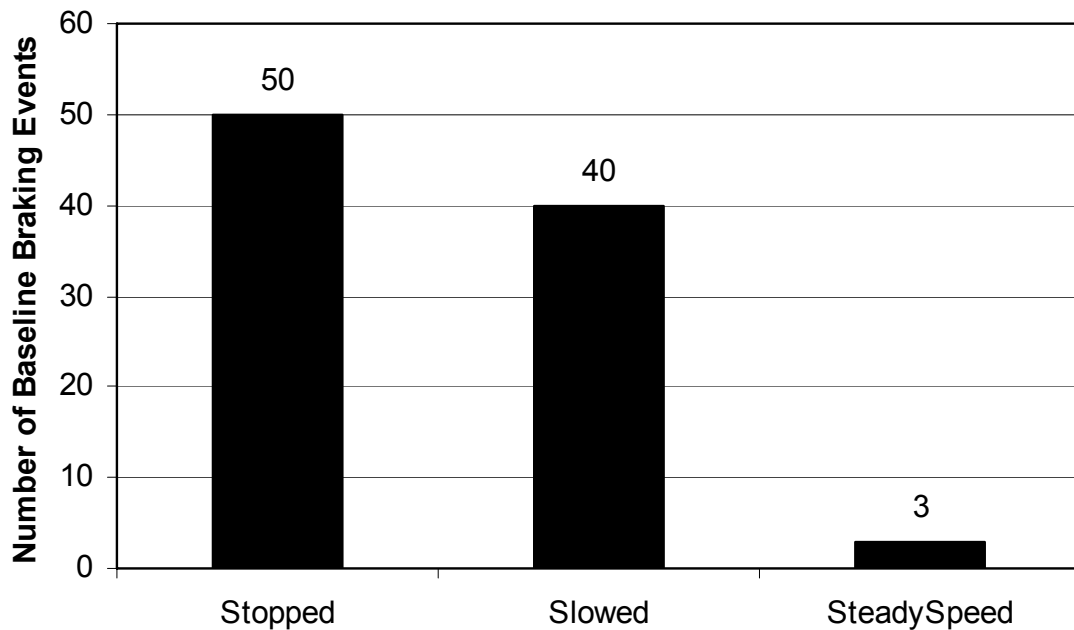
Figure 63. Disposition of baseline braking events with deceleration >0.7g .
