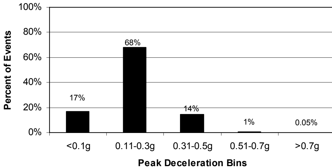
Figure 48. Percent of baseline braking events for various deceleration levels.
