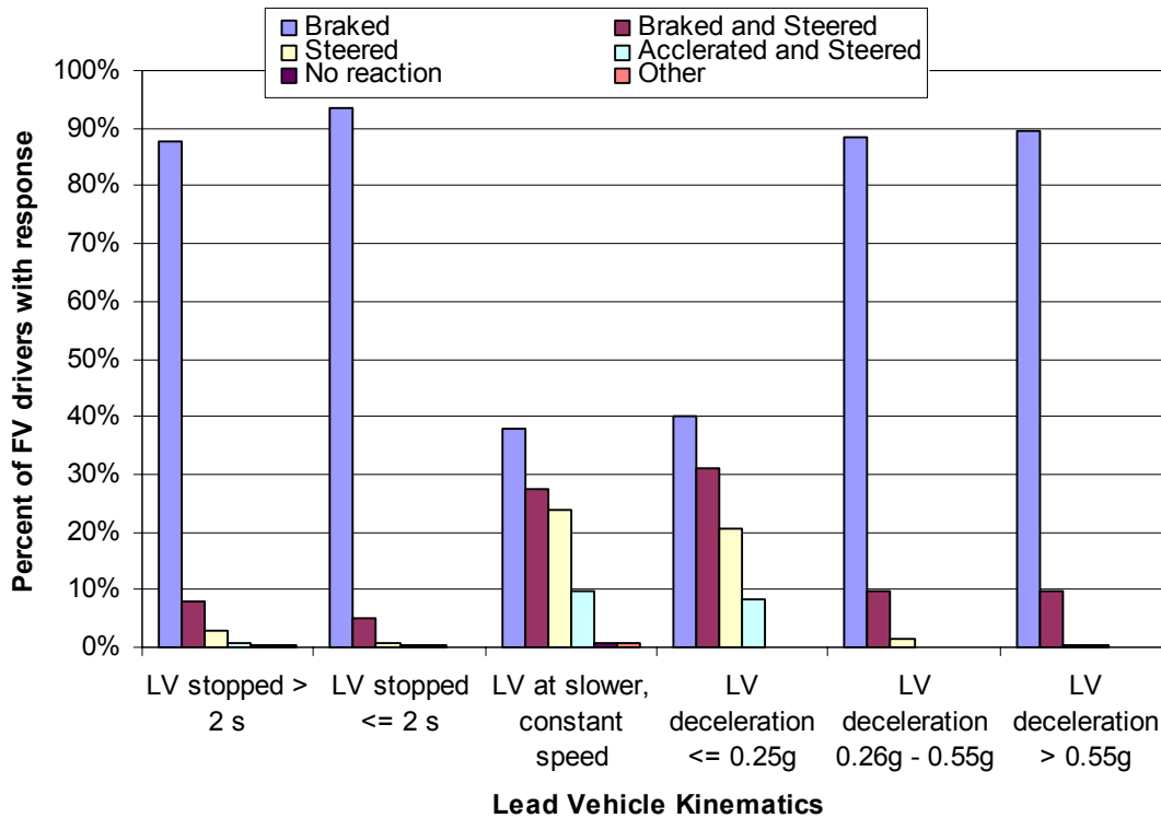
Figure 25. Percent of occurrence of FV-driver responses based on lead-vehicle kinematics scenarios.
