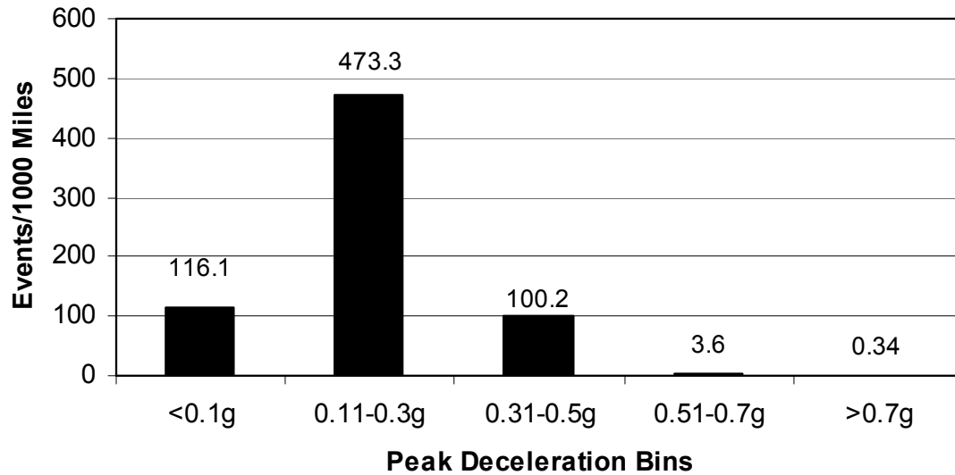
Figure 51. Number of baseline braking events per 1,000 miles of driving.
