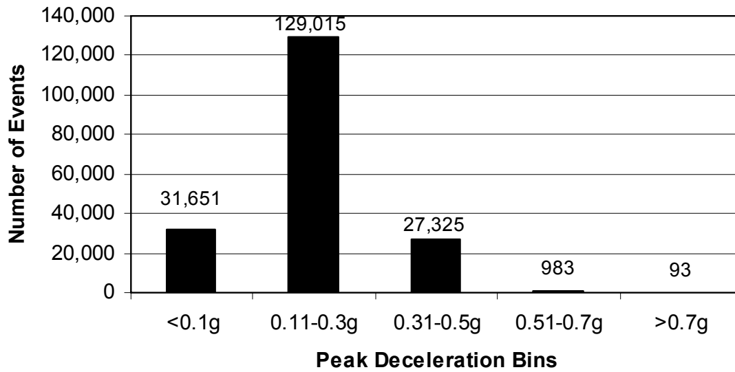
Figure 47. Number of baseline braking events for various deceleration levels.
