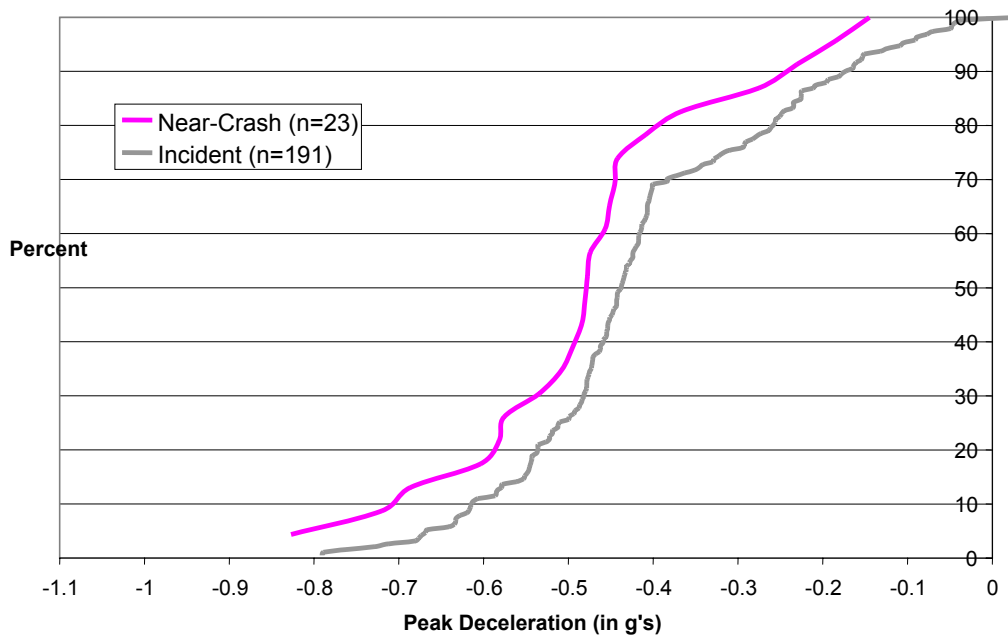
Figure 14. Lead-Vehicle Peak Deceleration, Near-Crash and Incident Events (Conflict with a Following Vehicle, Decelerating Lead).
