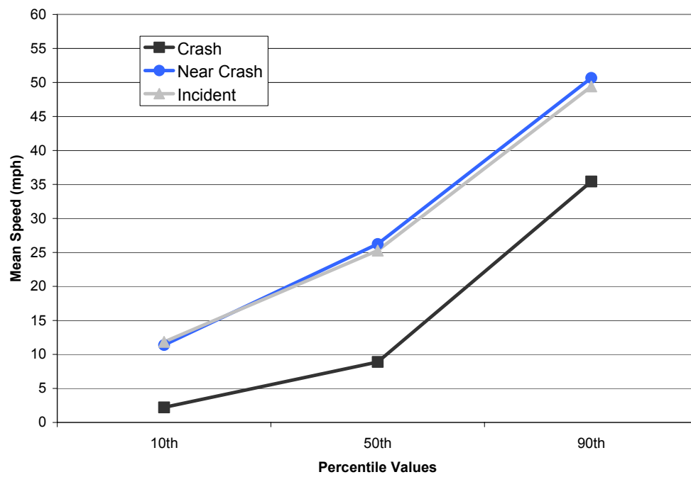
Figure 23. Percentile Values of Mean Speeds across Severity Levels (3 s before closest headway).
