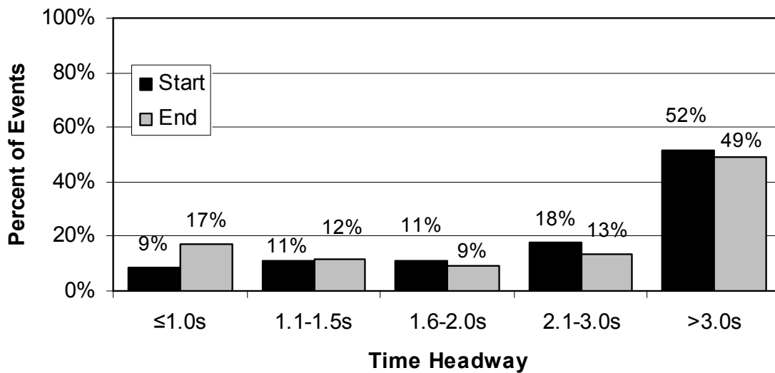
Figure 62. Percent of baseline braking events for various FV starting and ending headways.
