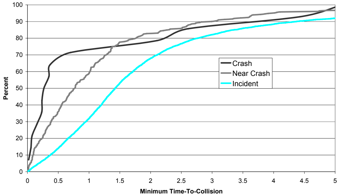
Figure 21. Distribution of Minimum TTC by Severity Level (3 s before closest headway).
