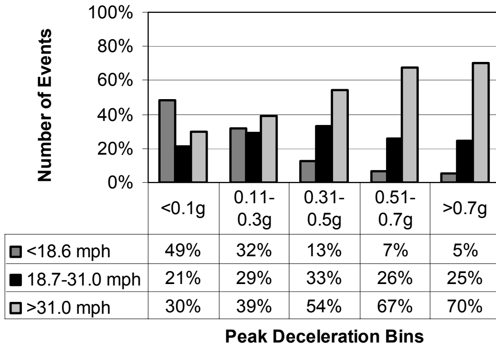
Figure 54. Distributions of various starting velocity categories for peak deceleration bins.
