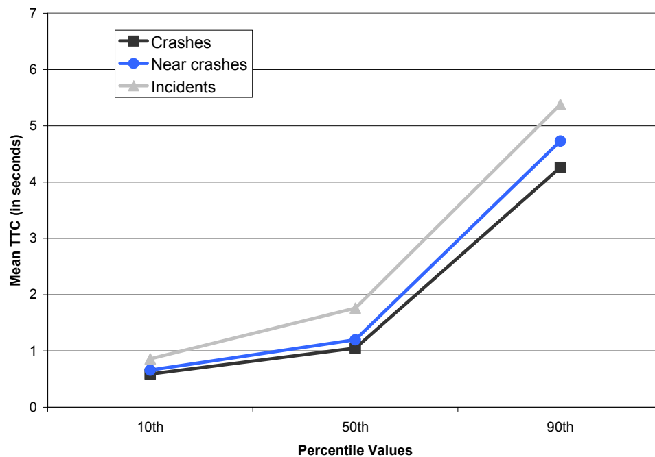
Figure 22. Mean TTC Percentile Values across Severity Levels (1 s before closest headway).
