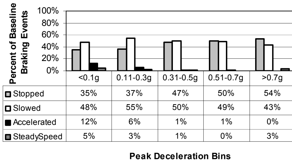
Figure 64. Distributions of various disposition categories for peak deceleration bins.
