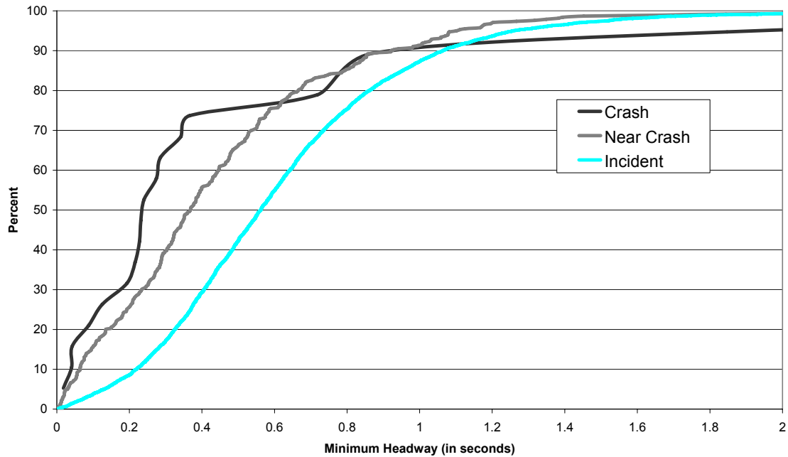
Figure 18. Distribution of Minimum Headways by Severity Level (1 s before closest headway).
