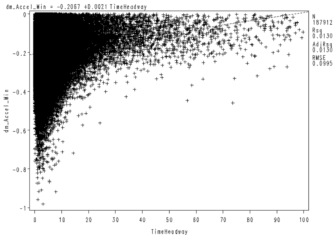
Figure 59. Linear regression plot of baseline braking events, with peak deceleration plotted against FV starting headway. The dashed line represents the line of best fit.
