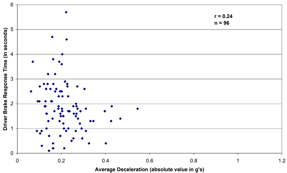
Figure 6. Scatterplot, brake-response time and average deceleration, near-crashes, conflicts with a decelerating lead vehicle.
