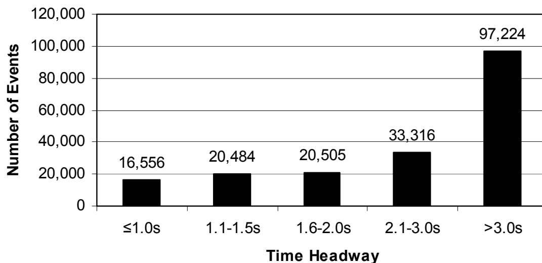
Figure 56 . Number of baseline braking events for various FV starting headways.
