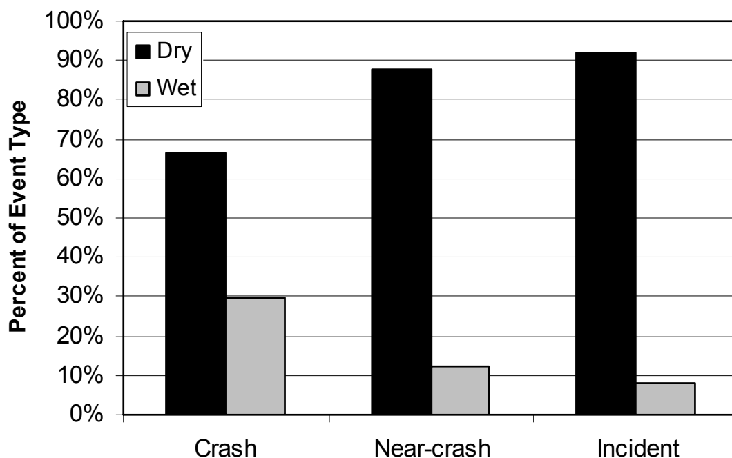
Figure 37. Percentage of Conflict With LV and Conflict With FV Events by Surface Condition.
