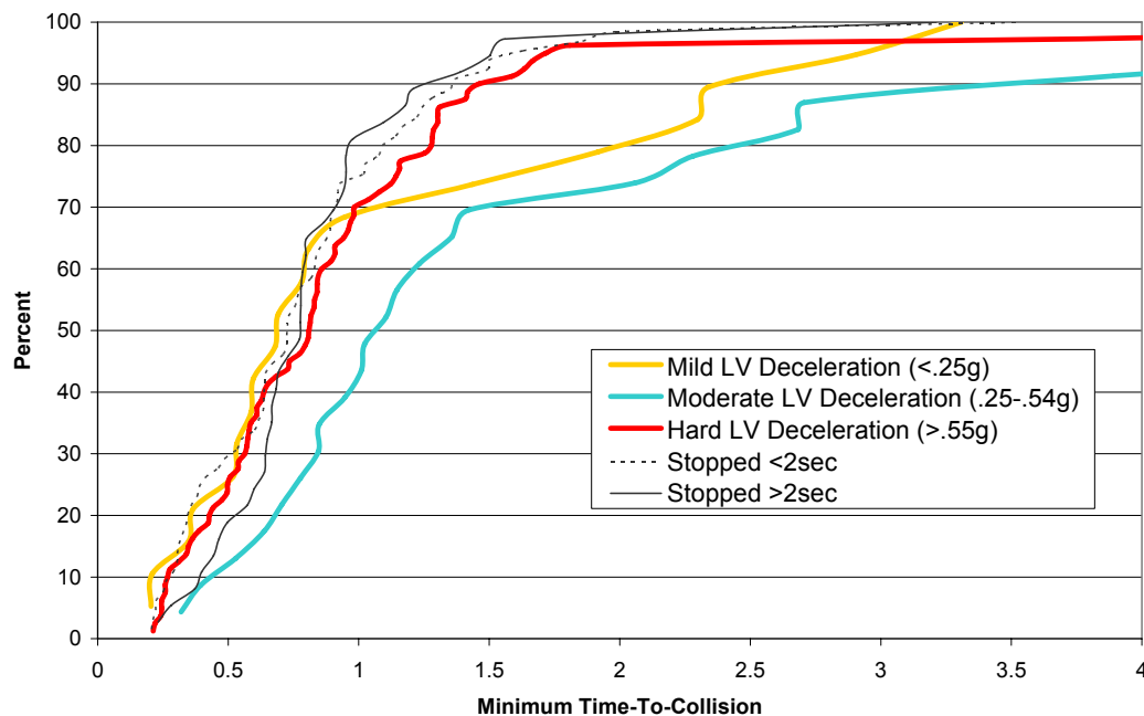
Figure 24. Distributions of Minimum TTC across Lead-Vehicle-Stopped/Deceleration Status (Near-Crashes, Conflicts with a Decelerating Lead Vehicle).
