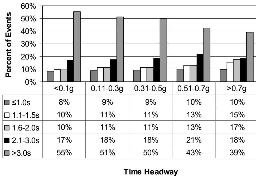
Figure 58. Distributions of various FV starting headway categories for peak deceleration bins.
