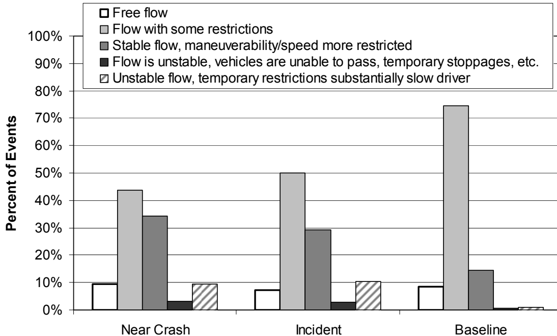
Figure 32. Distribution of traffic density conditions for near-crashes (N=32), incidents (N=320), and baseline events (N=1,102) occurring at intersection cluster locations.
