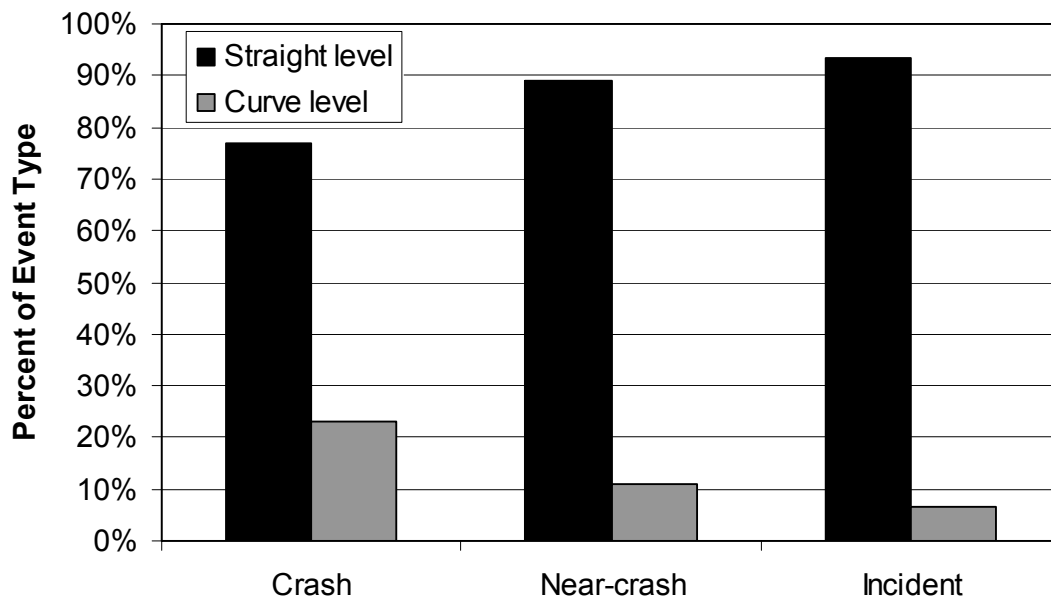
Figure 39. Percentage of Conflict With LV and Conflict With FV Events by Straight- and Curved-Road Alignment.
