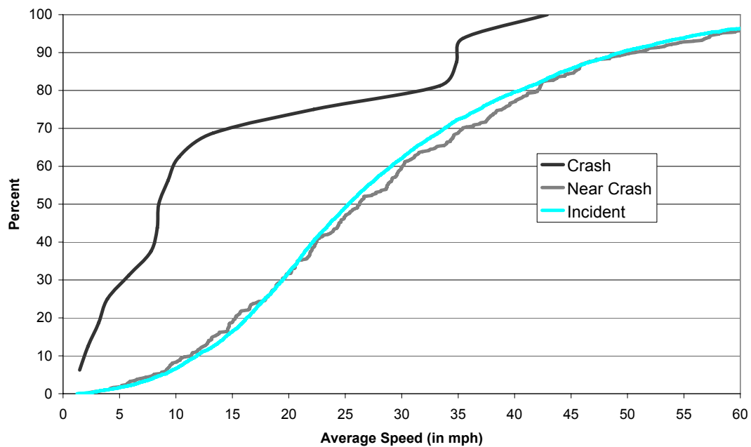
Figure 16. Distribution of Average Speed by Severity Level (1 s before closest headway).
