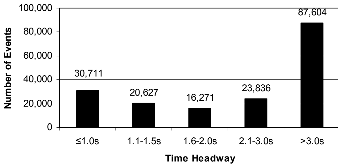
Figure 61. Number of baseline braking events for various FV ending headway.
