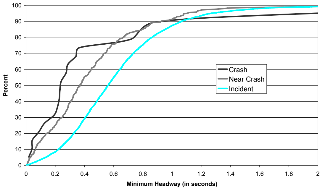
Figure 19. Distribution of Minimum Headways by Severity Level (3 s before closest headway).
