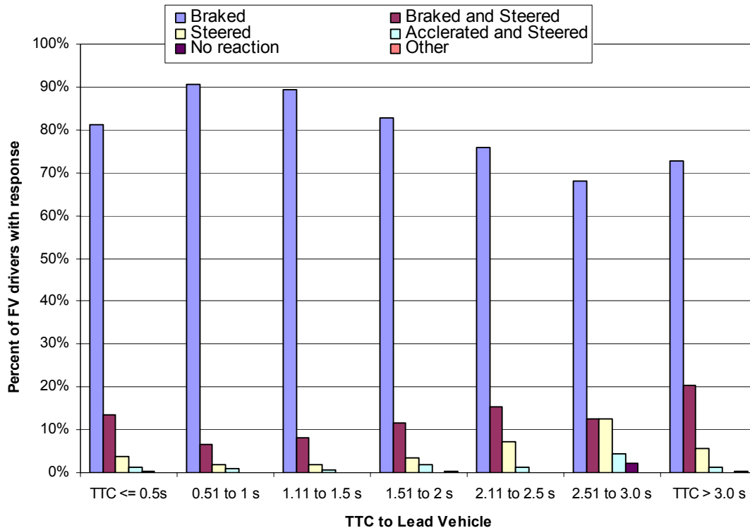
Figure 26. Percent of occurrence of FV-driver responses based on minimum TTC to lead vehicle.
