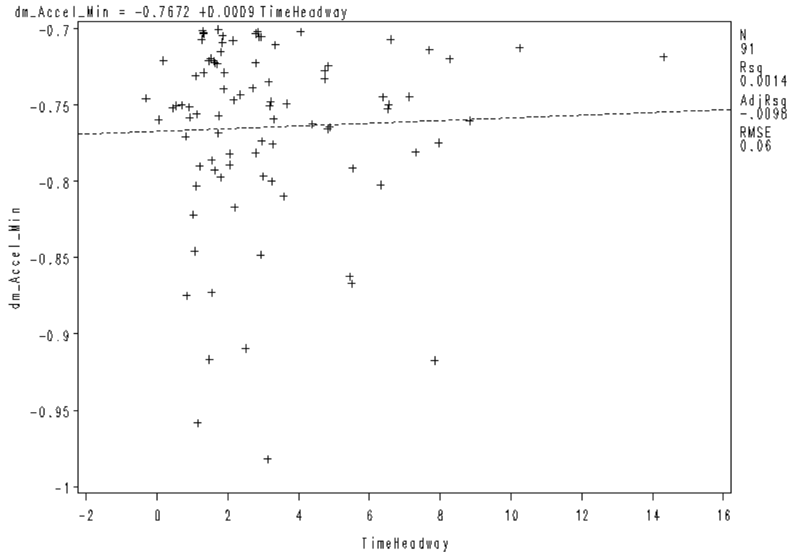
Figure 60. Linear regression plot of high deceleration baseline braking events, with peak deceleration plotted against FV starting headway. The dashed line represents the line of best fit.
