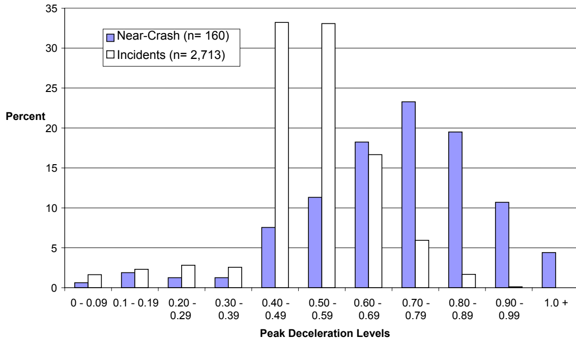
Figure 4. Peak deceleration categories, conflicts with a decelerating lead vehicle (near-crashes & incidents).
