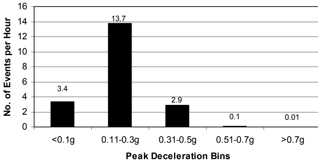
Figure 50. Number of baseline braking events per hour of driving.
