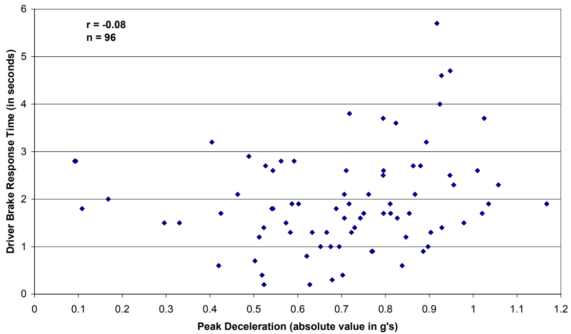
Figure 5. Scatterplot, brake-response time and peak deceleration, near-crashes, conflicts with a decelerating lead vehicle.
