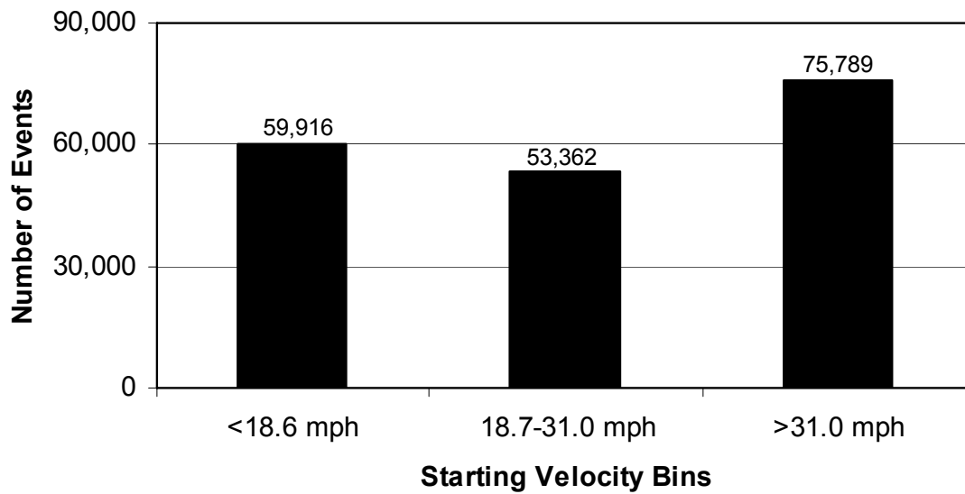
Figure 52. Number of baseline braking events for various starting velocities.
