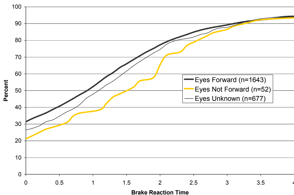
Figure 7. Distribution of brake-response times for incidents as a function of driver eye gaze at the onset of lead-vehicle braking (conflicts with a decelerating lead vehicle).
