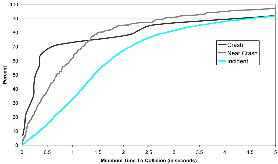
Figure 20. Distribution of Minimum TTC by Severity Level (1 s before closest headway).
