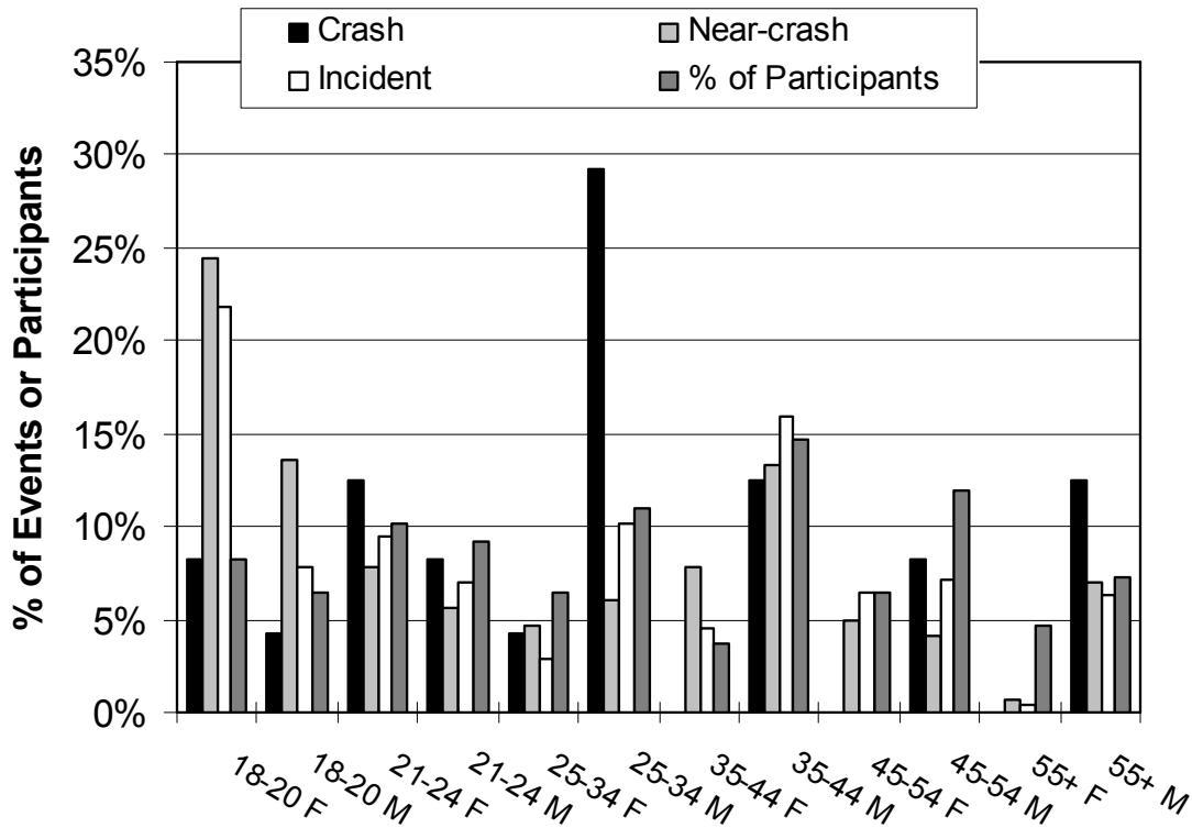
Figure 35. Age by Sex Distribution of Events for 100-Car Study Primary Drivers.
