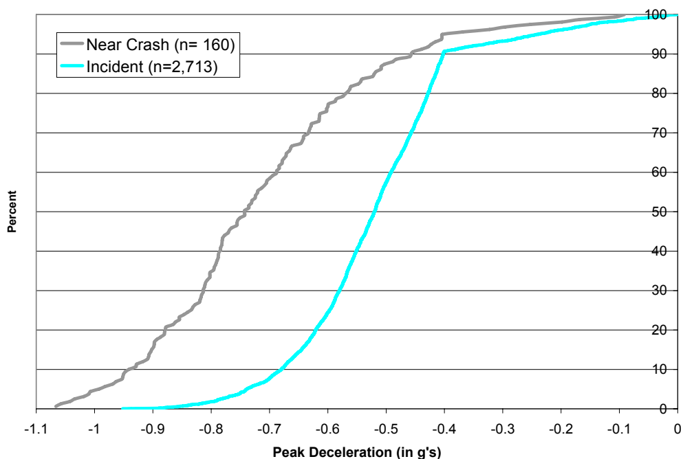
Figure 3. Cumulative distribution of peak deceleration, conflicts with a decelerating lead vehicle (near-crashes & incidents).
