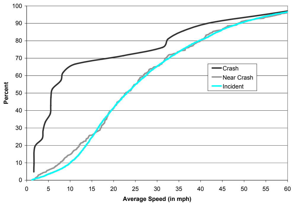
Figure 16. Distribution of Average Speed by Severity Level (1 s before closest headway).
