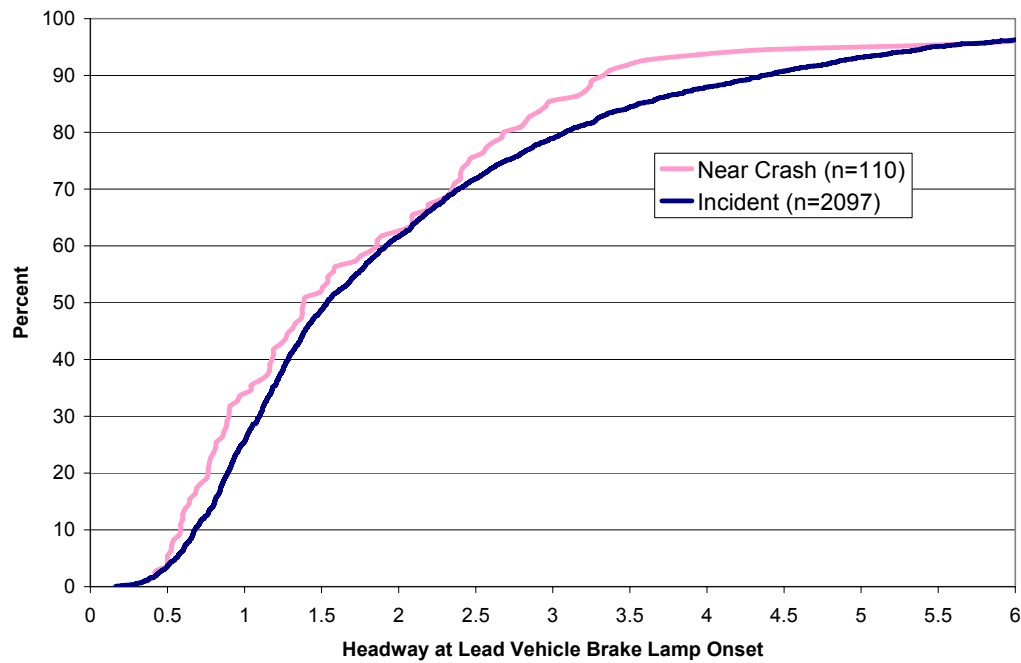
Figure 13. TTC (Seconds) at Onset of Lead-Vehicle Braking (Conflicts With a Lead Vehicle, Lead-Vehicle Decelerating Cases).
