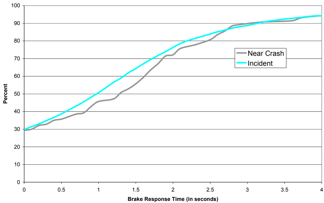
Figure 1. Cumulative distribution of brake-response times, conflicts with a decelerating lead vehicle (near-crashes & incidents).
