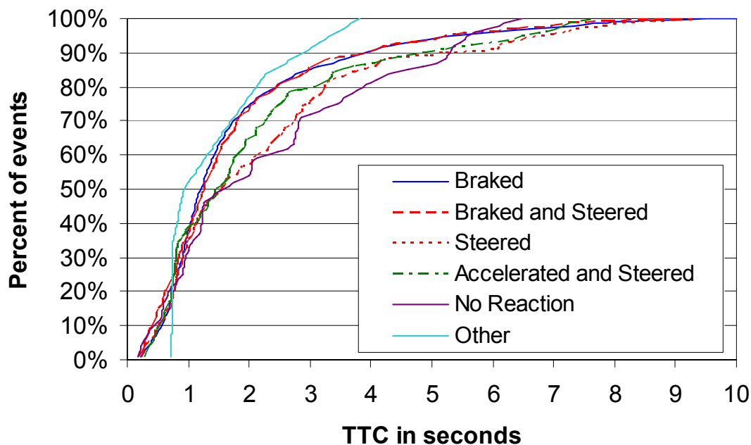
Figure 27. Distribution of FV-driver responses based on minimum TTC to lead vehicle.
