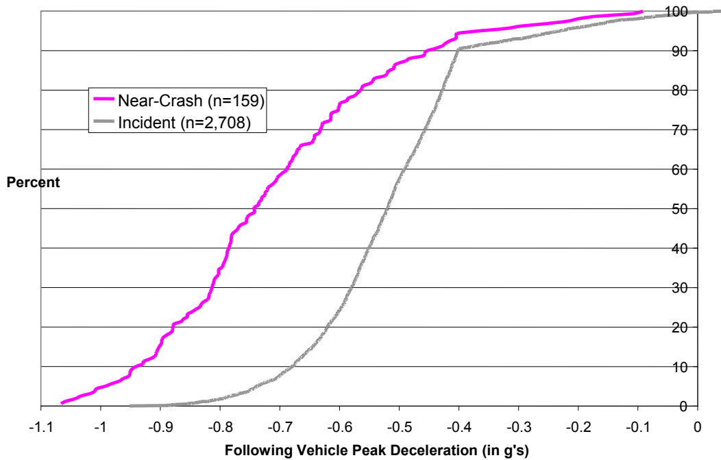
Figure 15. Following-Vehicle Peak Deceleration by Severity Level (Conflict With a Lead Vehicle, Lead-Vehicle Decelerating).
