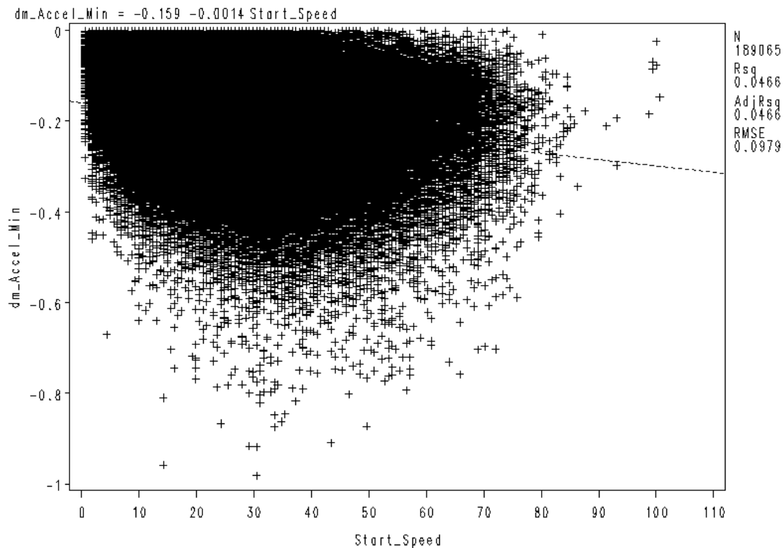
Figure 55. Linear regression plot of baseline braking events, with peak deceleration plotted against starting velocity. The dashed line represents the line of best fit.
