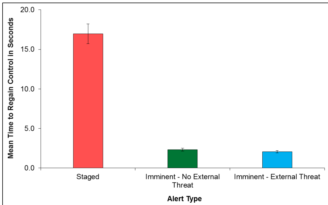
Figure 4-12. Time to Regain Control, Stratified by Alert Type, After the Onset of the Alert
